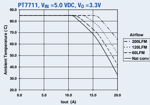
Safe Operating Area Curves (Note B)
